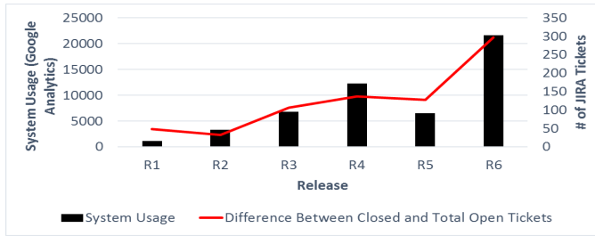
Figure 1. Impact of software maintenance effort on system usage.
