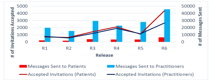
Figure 3. Service usage/activity triggers activities based on customer type.
