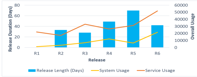
Figure 2. System usage versus release duration.
