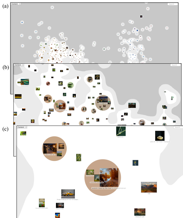
Figure 5: When zooming into the content map from (a) to (c), the base layer gets gradually magnified and the items, here photographs, are appropriately filtered and displayed with more detail.
