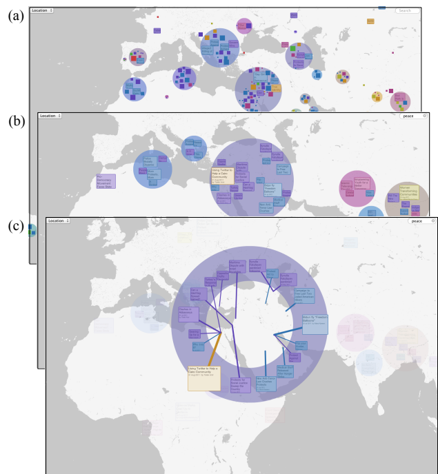
Figure 11: Looking for ‘peace’ in blog articles about the Middle East, North Africa, and South Europe.
