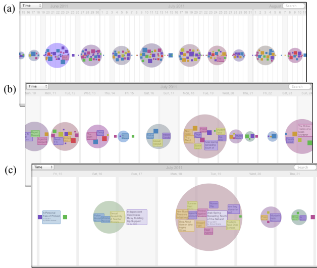
Figure 3: The time scale is changed from (a) two months, to (b) two weeks, and (c) seven days.
